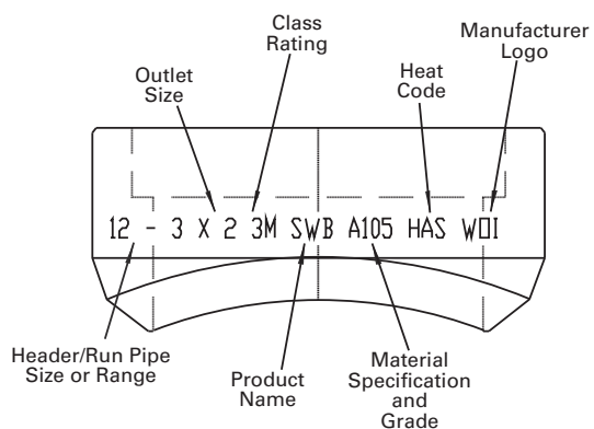
Socket Weld Branchette™ (SWB)
