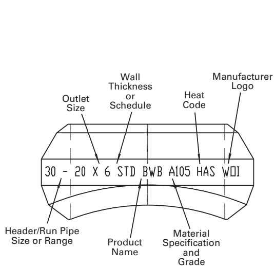
Buttweld Branchette™ (BWB)
