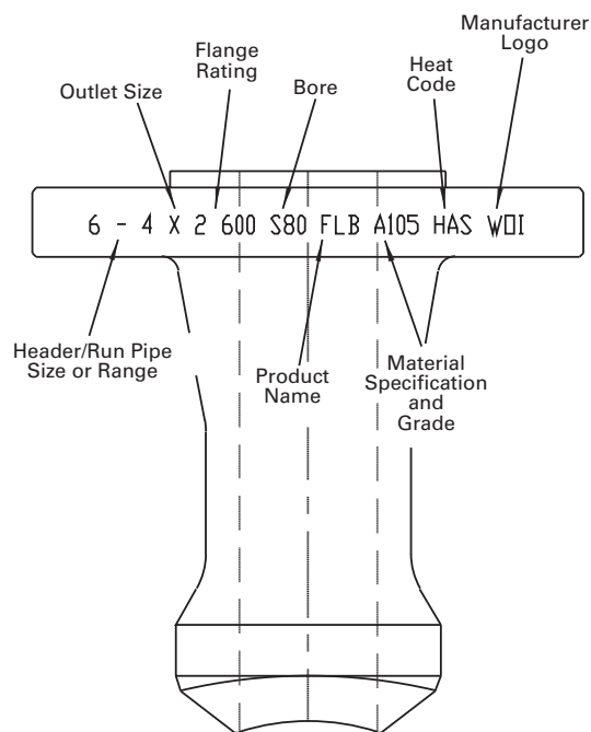
Flanged Branchette™ (FLB)
