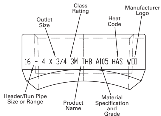
Threaded Branchette™ (THB)
